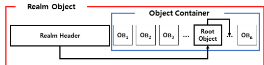
Fig. 1. Realm Object Structure
